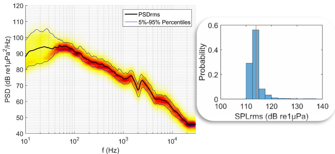
Fig. 3.1.2. Aggregated 30 sec PSDs concerning Lefkada station and SPLrms histogram (bin width 2.5 dB re 1 μPa) with average value indication.
