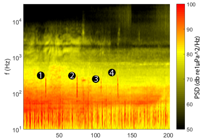
Fig. 3.2.8. PSD spectrogram indicating the four impulsive sounds detected in Paxoi station on February 6 th .
