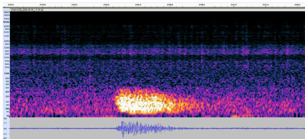
Fig. 3.2.10. PSD spectrogram of the 2 nd impulsive sound detected in Paxoi station on February 6 th . It reaches SPLp-p = 150 dB re 1 \mu Pa, while the mean ambient noise is around 130 dB (20 dB increase).
