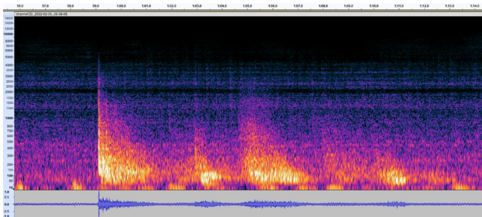
Fig. 3.2.6. PSD spectrogram of the 1 st impulsive sound detected in Lefkada station on February 6 th . It is composed of a loud main impulse followed by at least 4 echoes. The main impulse reaches SPL p-p = 155 dB re 1 μPa, while the mean ambient noise is around 135 dB (20 dB increase).
