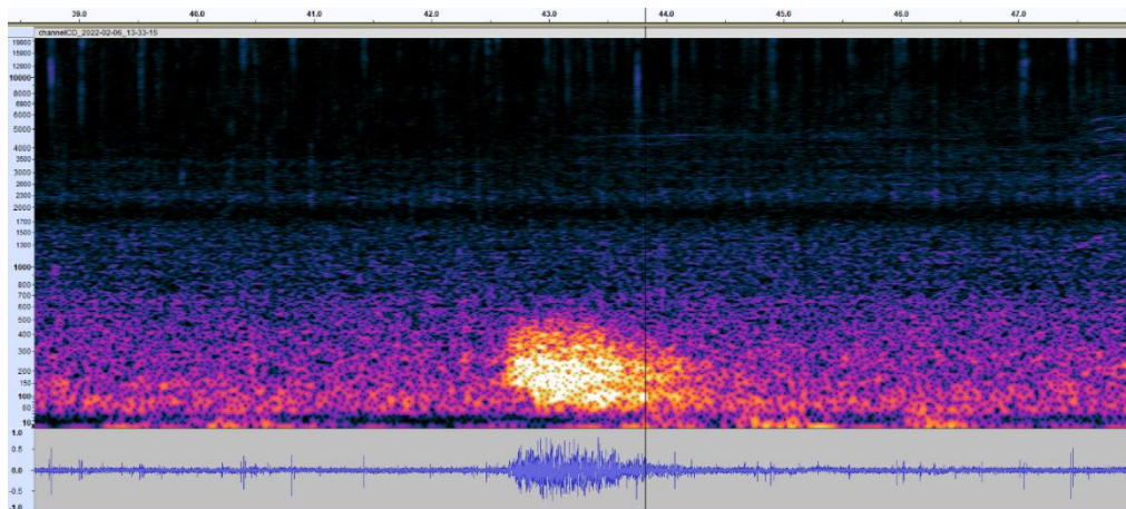
Fig. 3.2.12. PSD spectrogram of the 4 th impulsive sound detected in Paxoi station on February 6 th . It reaches SPL p-p = 140 dB re 1 \mu Pa, while the mean ambient noise is around 140 dB (10 dB increase).
