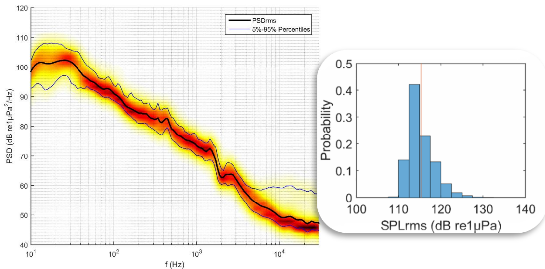
Fig. 3.1.6. Aggregated 30 sec PSDs concerning Kerkyra South station and SPLrms histogram (bin width 2.5 dB re 1 μPa) with average value indication.
