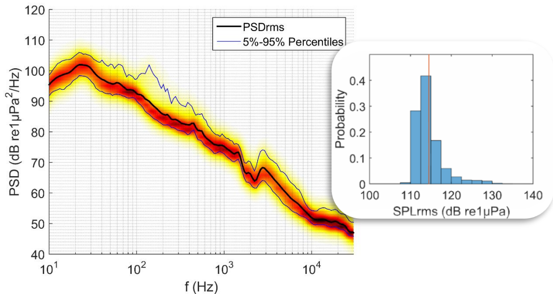
Fig. 3.1.8. Aggregated 30 sec PSDs concerning Kerkyra North station and SPLrms histogram (bin width 2.5 dB re 1 μPa) with average value indication.
