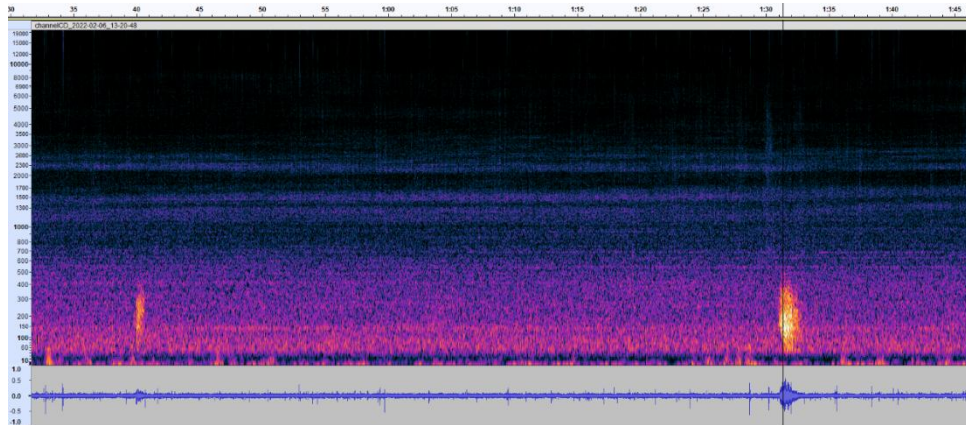
Fig. 3.2.11. PSD spectrogram of the 3 rd impulsive sound detected in Paxoi station's PSD on February 6 th . It actually consists of two impulses, with the last and louder impulse reaching SPL p-p = 150 dB re 1 \mu Pa, with the mean ambient noise being around 140 dB (10 dB increase) and the first being of less that 5dB louder and concentrated on very low frequencies.
