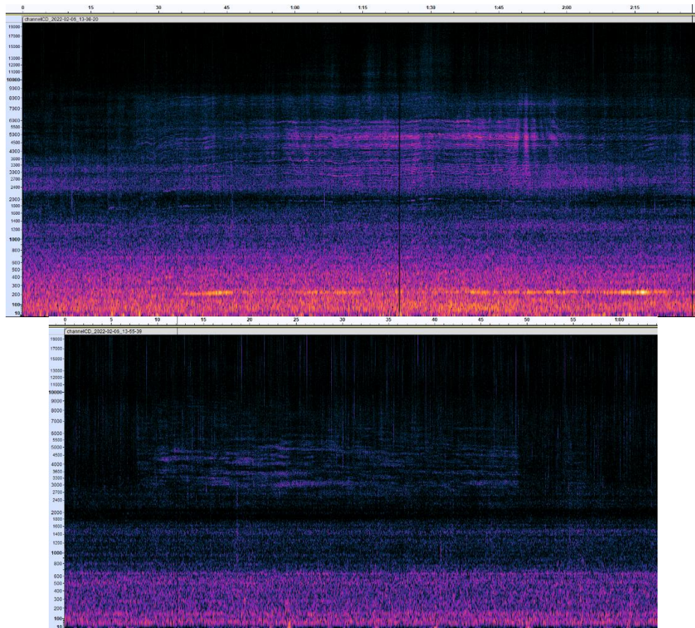
Fig. 3.2.4. PSD spectrograms for traffic noise evident in the ambient sound recordings of Paxoi station, regarding fishing vessels passing around 1nm away.
