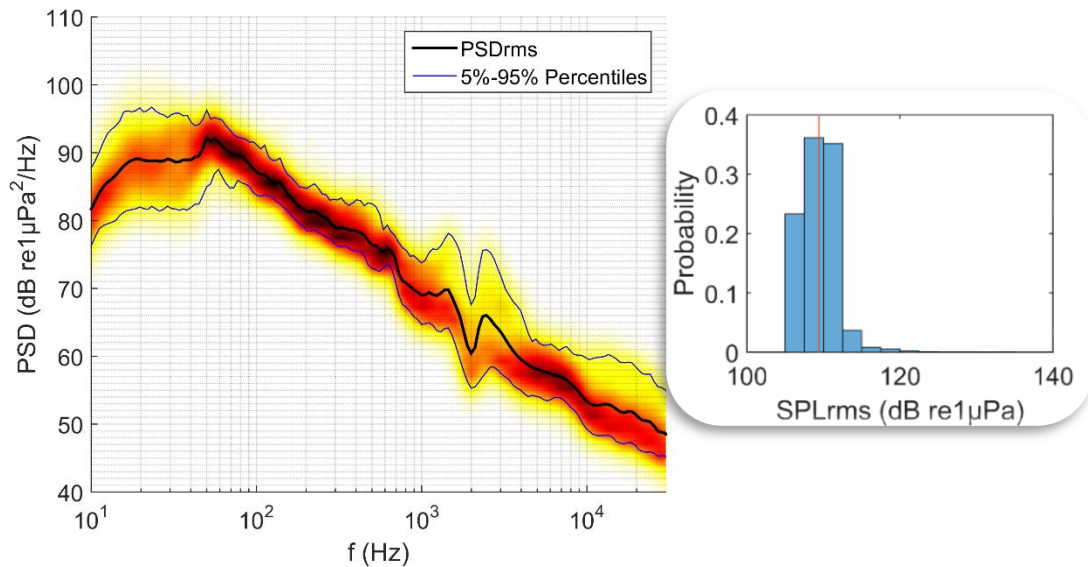
Fig. 3.1.4. Aggregated 30 sec PSDs concerning Paxoi station and SPLrms histogram (bin width 2.5 dB re 1 μPa) with average value indication.
