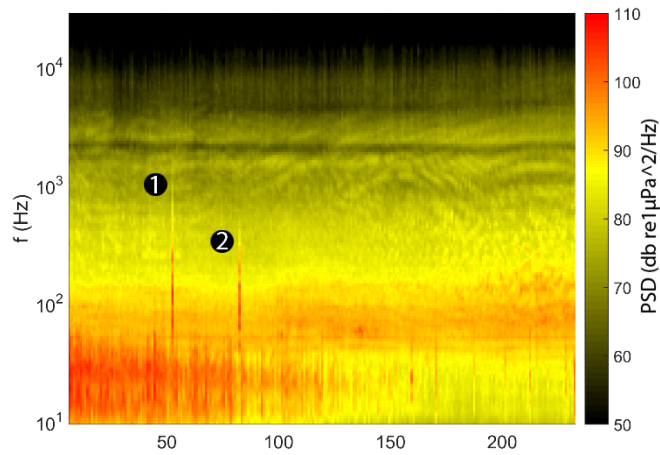
Fig. 3.2.5. PSD spectrogram indicating the two impulsive sounds detected in Lefkada station on February 6 th .
