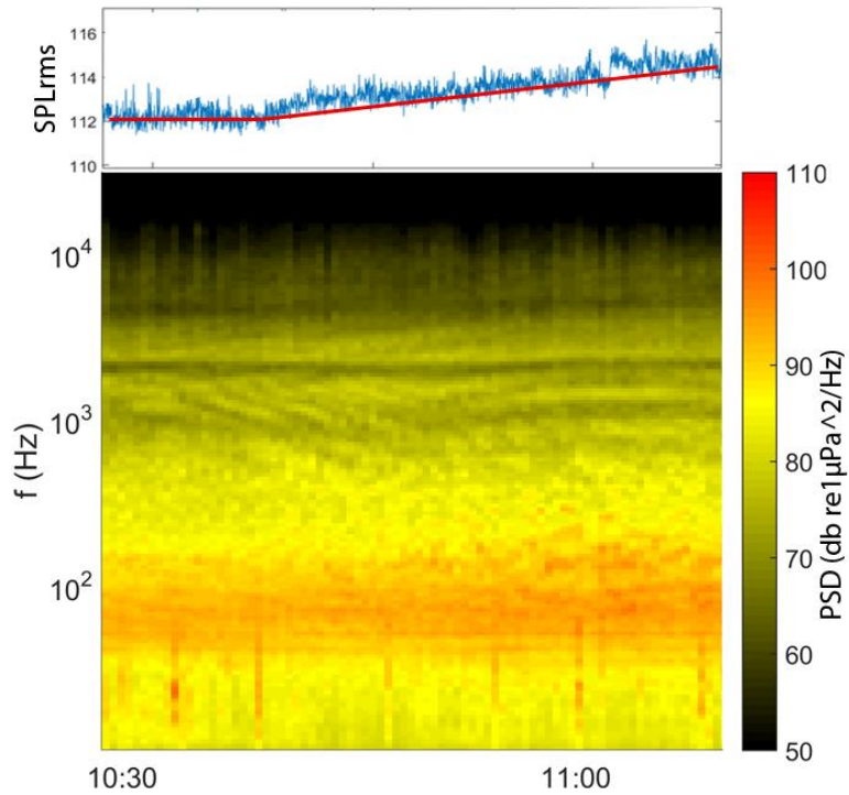
Fig. 3.2.2 SPLrms and PSD spectrogram for traffic noise evident in the sound recording of Lefkada station on February 6th, indicating a fishing vessel 6 nm away.
