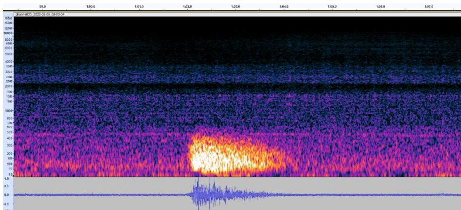
Fig. 3.2.7. PSD spectrogram of the 2 nd impulsive sound detected in Lefkada station on February 6 th . It reaches SPL p-p = 155 dB re 1 μPa, while the mean ambient noise is around 135 dB (20 dB increase).
