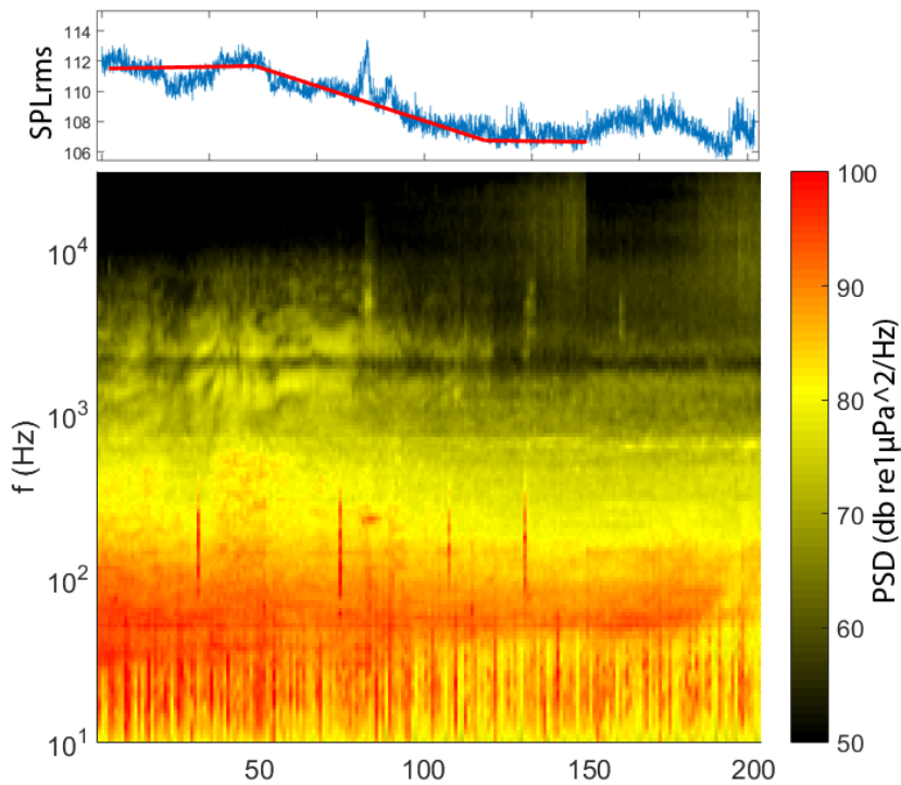
Fig. 3.2.3 SPLrms and PSD spectrogram for traffic noise evident in the sound recording of Lefkada station on February 6th, indicating a Cargo ship 10nm away.
